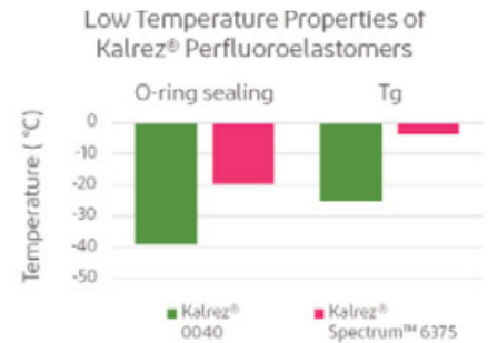
Low temperature static sealing (DuPont Proprietary test method)
