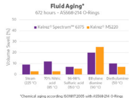
Kalrez® MS220 vs Kalrez® Spectrum 6375 Chemical resistance
