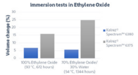
Kalrez® Spectrum™ 6380 weight change in Ethylene Oxide (still the preferred Kalrez® option for Ethylene Oxide / Water mix)
